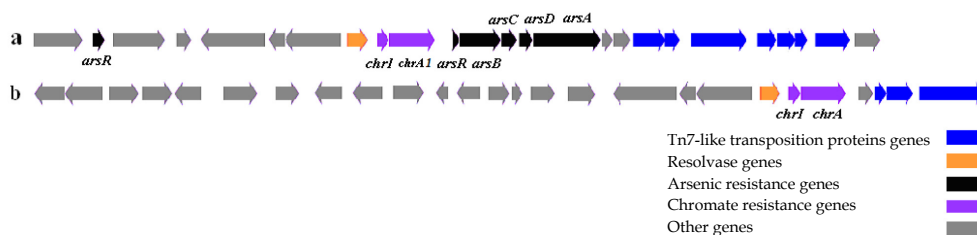
Fig. 3. Comparison of genetic determinants of chromate resistance and chromate reduction between (a) Bacillus cereus SJ1 and (b) Bacillus thuringiensis serovar konkukian str. 97-27. (After He et al. , 2010).
